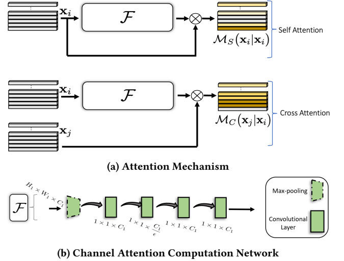
Figure 3: Proposed Attention Module. (a) Self-Attention (top) on latent representation \mathbf{x}_i and Cross-Attention (bottom) for representation \mathbf{x}_j conditioned on \mathbf{x}_i . Symbol \otimes denotes element-wise multiplication of each attention weight with respective channel of the representation. (b) The channel weight computation function \mathcal{F} . It generates channel descriptor by channel-wise global average pooling to learn attention weights for each channel.
